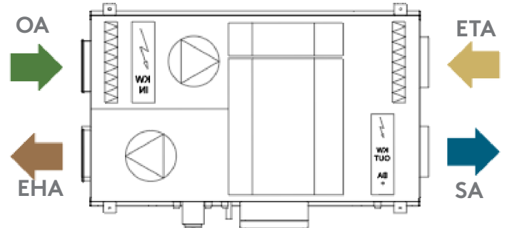
GLOBAL PX LP 02 - 10/14 - 18 (Top view)
