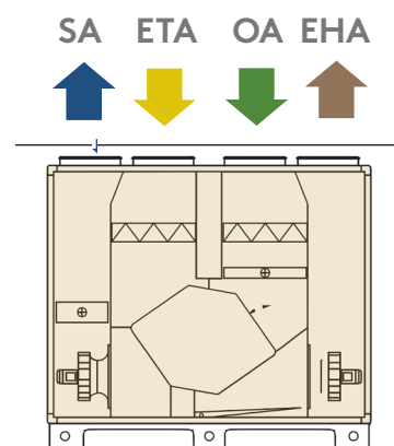
GLOBAL PX LP 02 - 10/14 - 18 (Top view)
