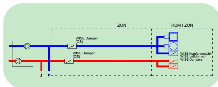
Principskiss, Positionsoptimering
