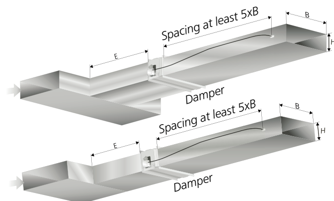
Figure 7. Requirements for straight duct section and distance in rectangular ducts. E = Straight section B = Width of duct H = Height of duct
