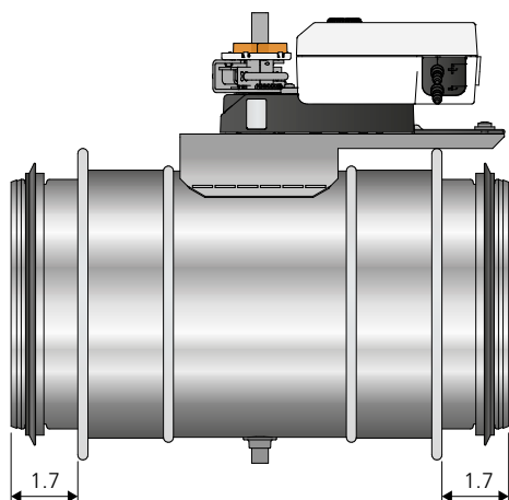
Figure 2. Dimensions (in), REACT P GMB circular with DUCT ADAPTER installed.
