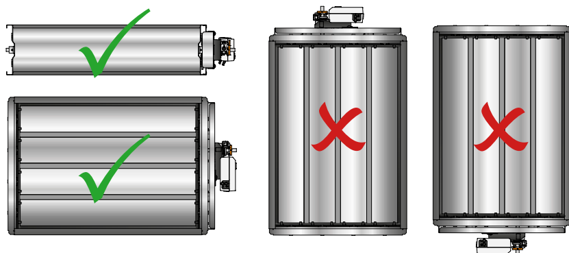
Figure 6. Installation - For rectangular ducts, always install the damper so that the controller/actuator is placed along the side of the duct.
