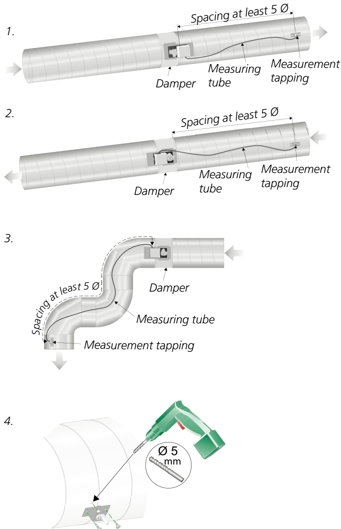
Figure 4. Installation in the duct system. The ducts must be firmly fixed to the frame of the building on each side of the product.
