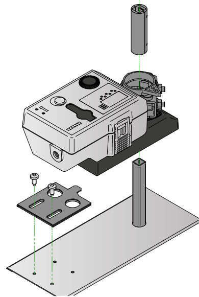
Figure 12. Dismantling the damper motor.
