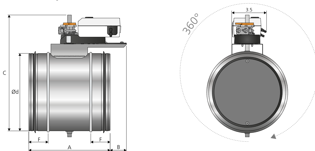
Figure 1. Dimensions (in), REACT P GMB circular. The damper can be installed at an optional angle.
