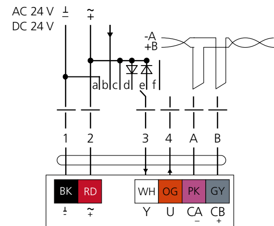
Figure 8. Wiring diagram.
