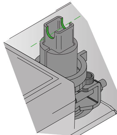
Figure 13. Recess in the damper shaft indicates the position of the damper.
